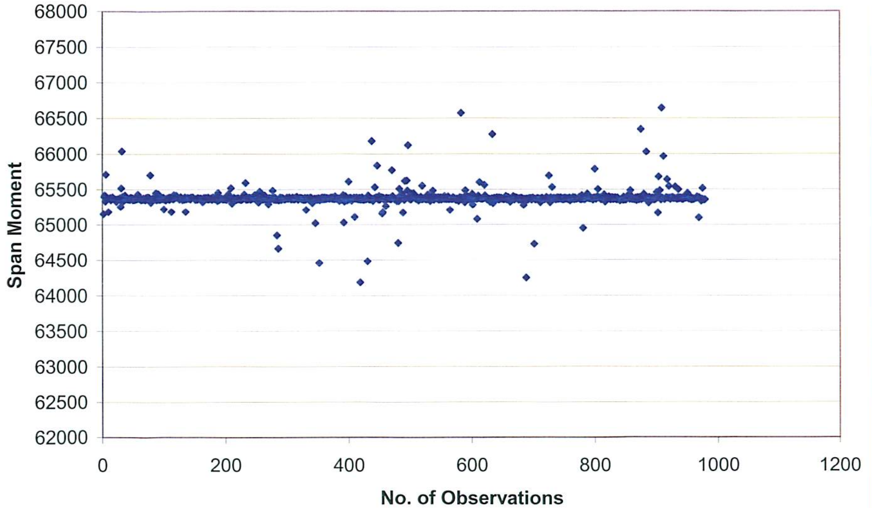
CH-47 Span Moment (after balancing)
